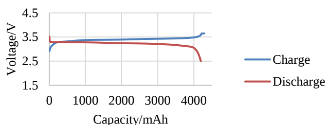
JGCFR26650-4000mAh-3.2V Charge-Discharge curves(0.2C)
