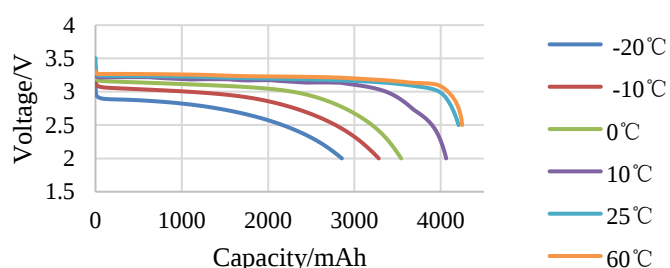
JGCFR26650-4000mAh-3.2V Discharge curves at different temperature(0.5C)
