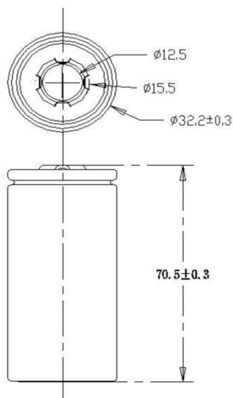
电池图片和外形尺寸 Cell's appearance and dimension
