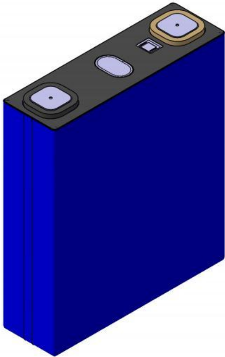
13.2电芯尺寸图Cell Dimension Drawing
