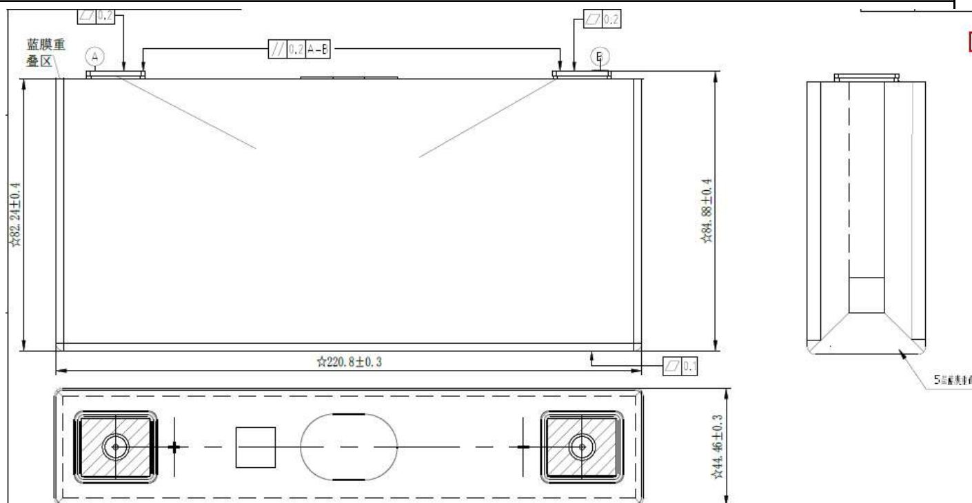
二维图纸 2D Drawing
