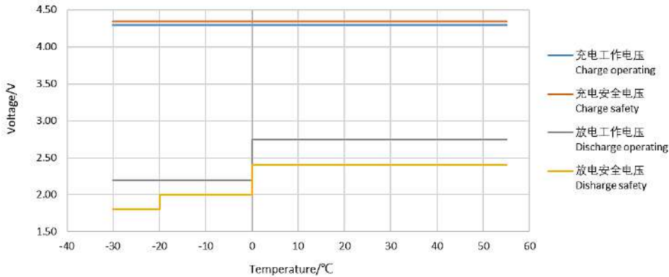
工作电压与安全电压限制 Operating and Safety Voltage Limit
