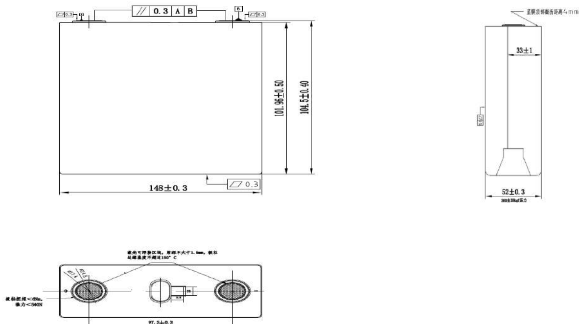
二维图纸 2D Drawing
