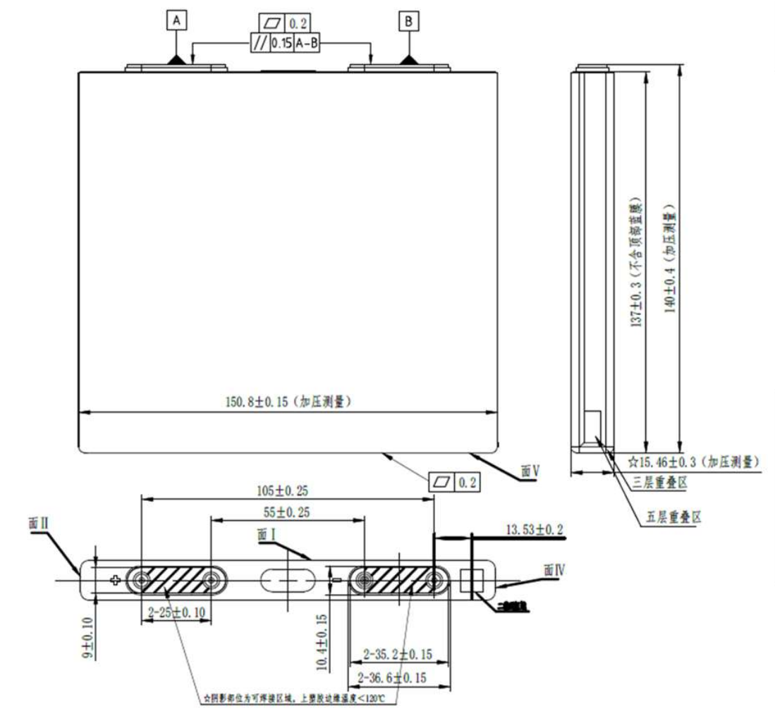
二维图纸 2D Drawing
