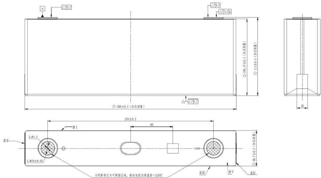
二维图纸 2D Drawing
