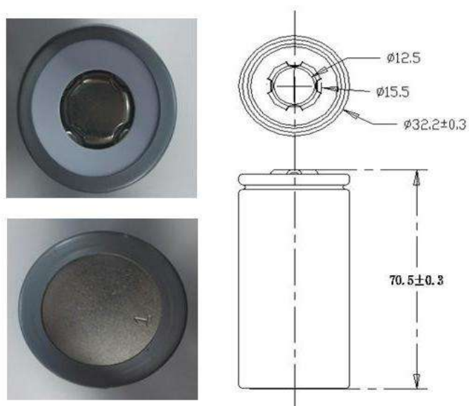
电池图片和外形尺寸 Cell's appearance and dimension
